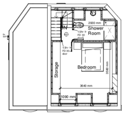
1 Proposed Second Floor 1:100
