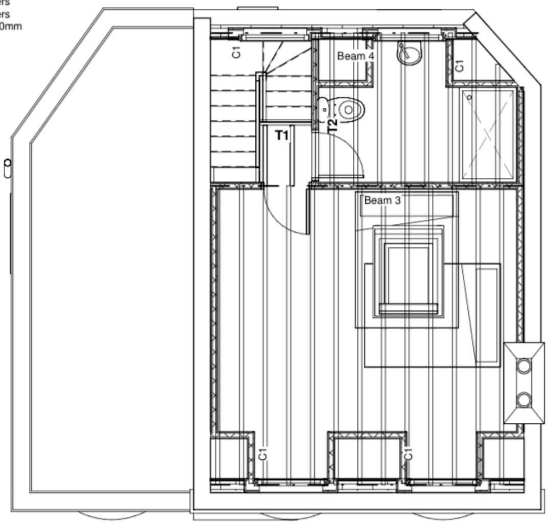
1 Proposed Second Floor 1:100
