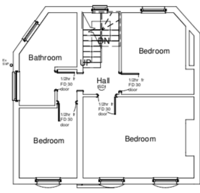
2 Proposed First Floor 1:100
